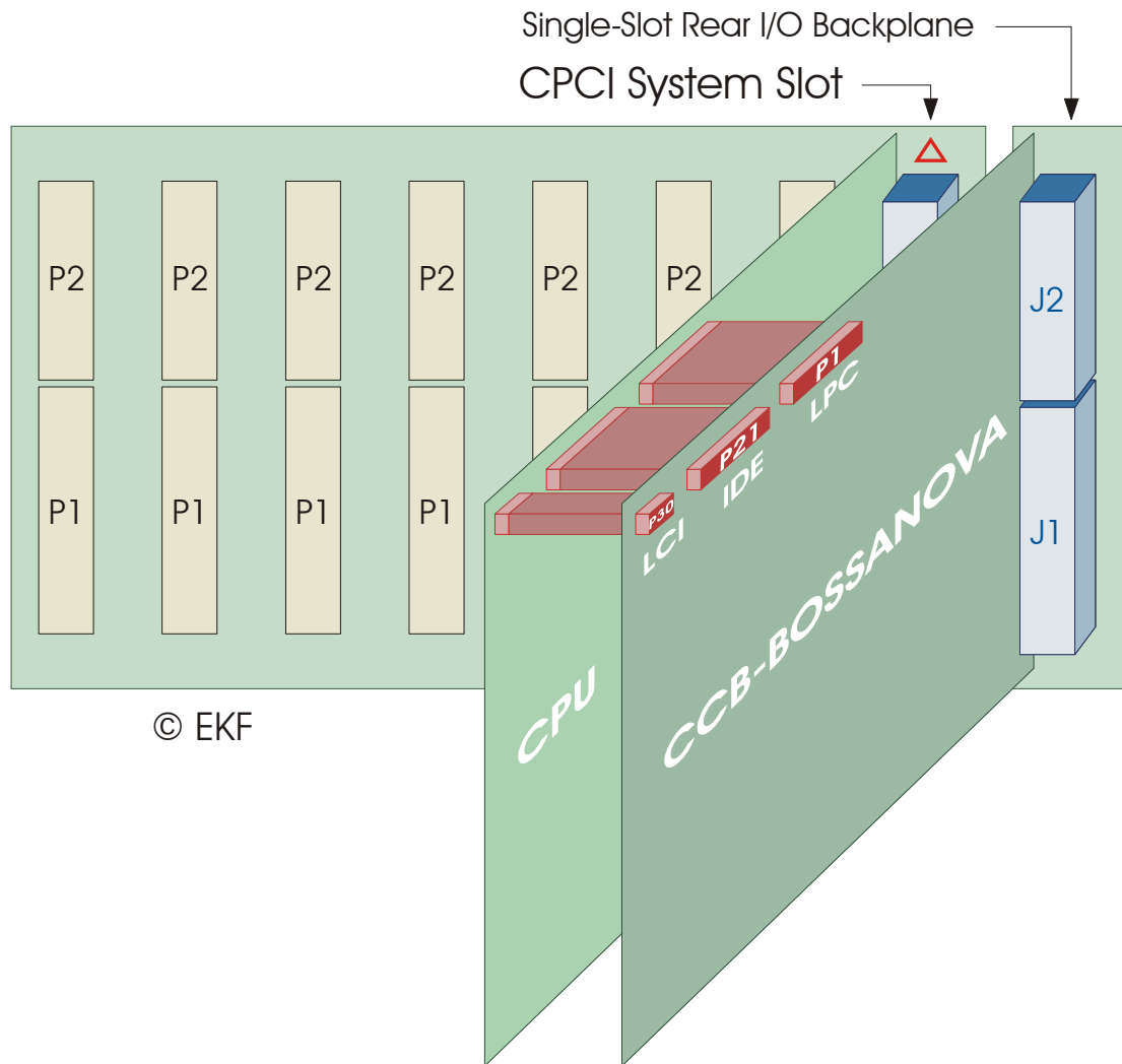
CCB-BOSSANOVA mounted on top of the CPU carrier board
