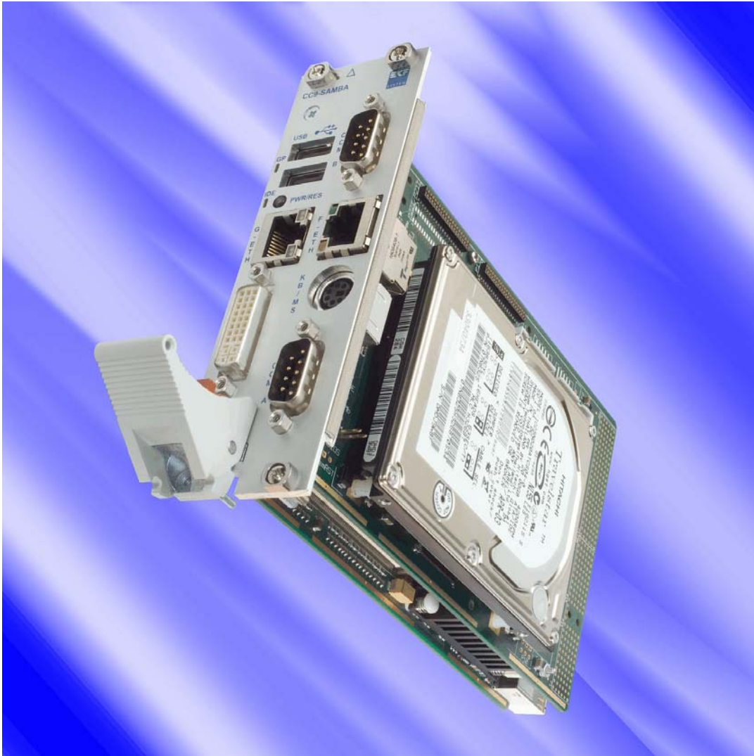
CCB-2-BOSSANOVA with Hard Disk Option
