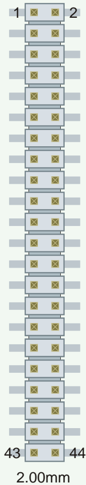
P24 On-Board 2.5-Inch Hard Disk Drive 2.00mm Pin Header 2x22
