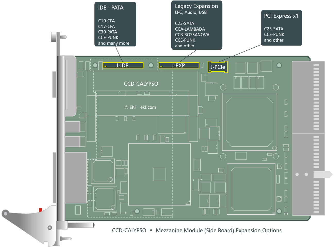
Mezzanine Connectors on a CPU Carrier Board
